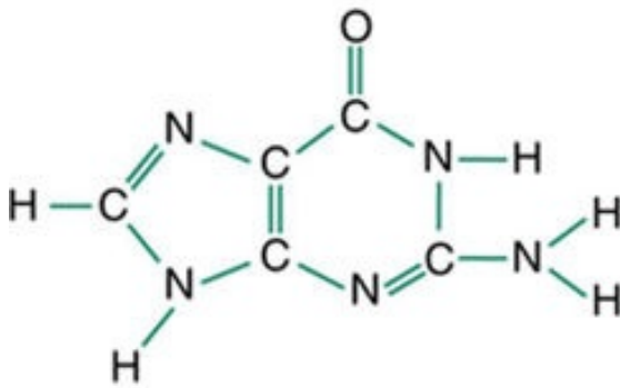
Guanina
