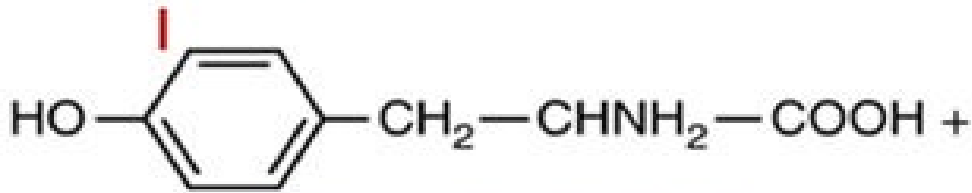
Monoyodotirosina
