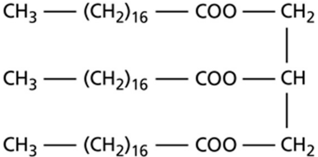
Triestearina
