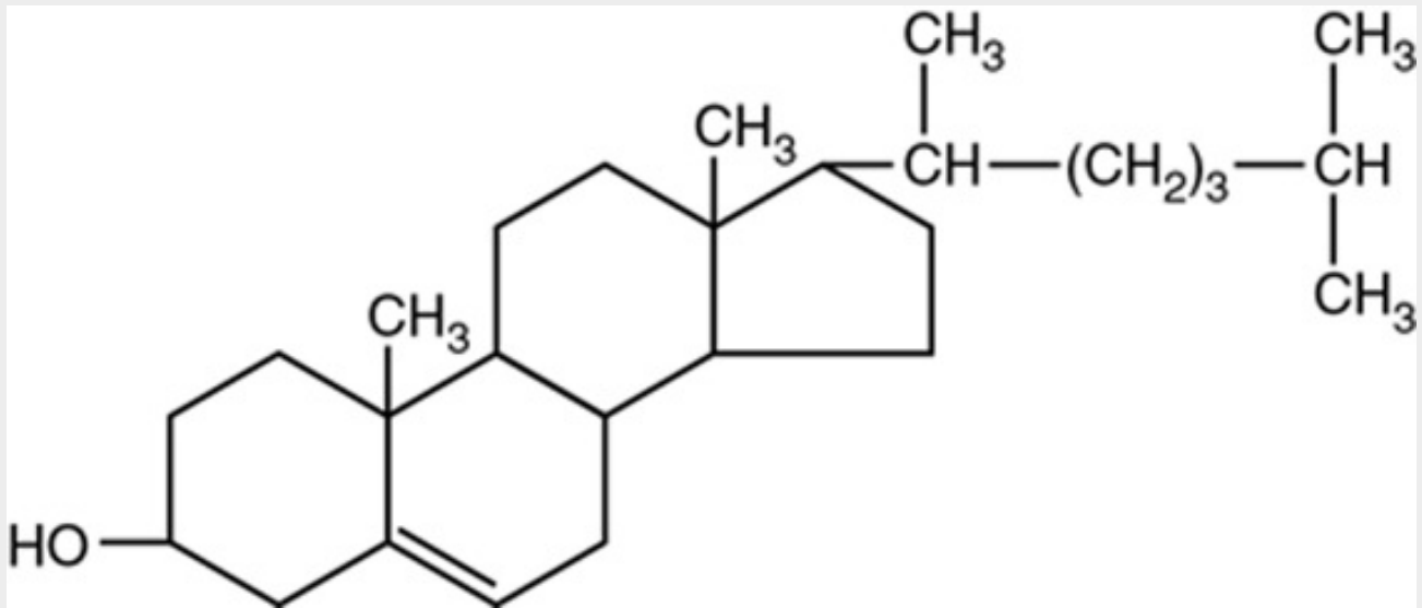
FIGURA 69-6 Colesterol.
